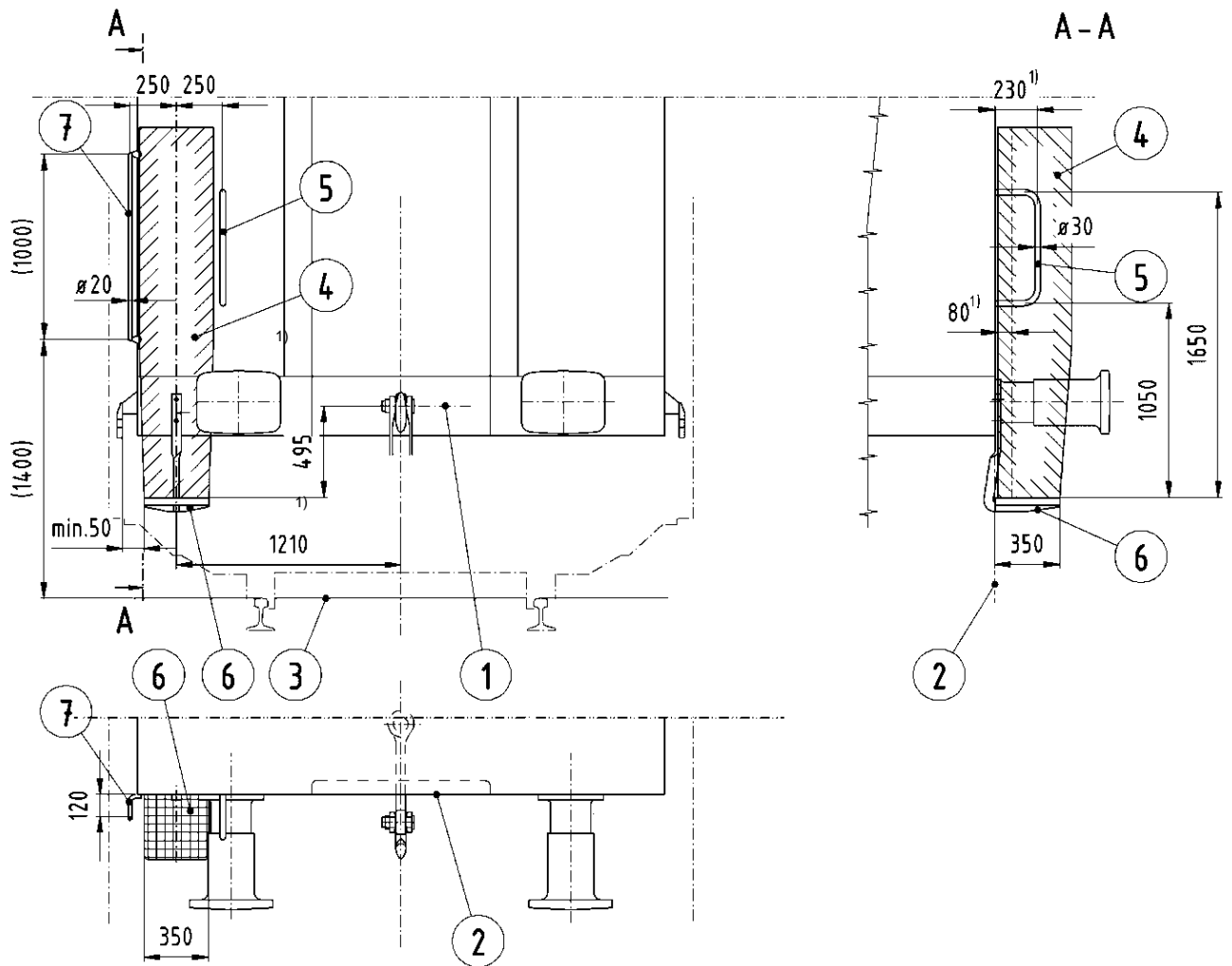
Figure 5: Shunter's stand
