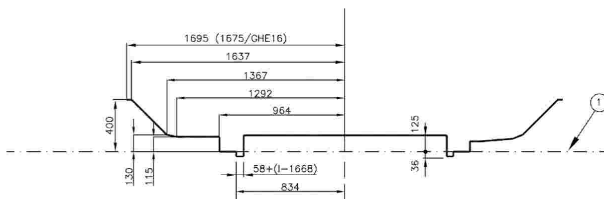
Figure 12 Reference profile of lower parts of kinematic gauge GEI1 for vehicles which can pass over rail brakes in an active position (l = track gauge) (Dimensions in millimeters)
