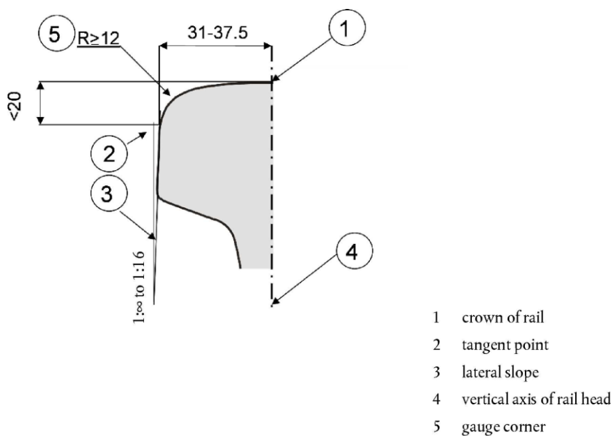
Figure 1 Railhead profile
