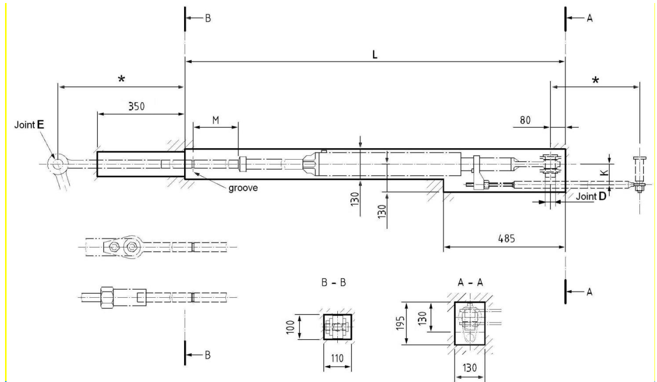
Figure 2: Space envelope for loads greater than 75 kN
