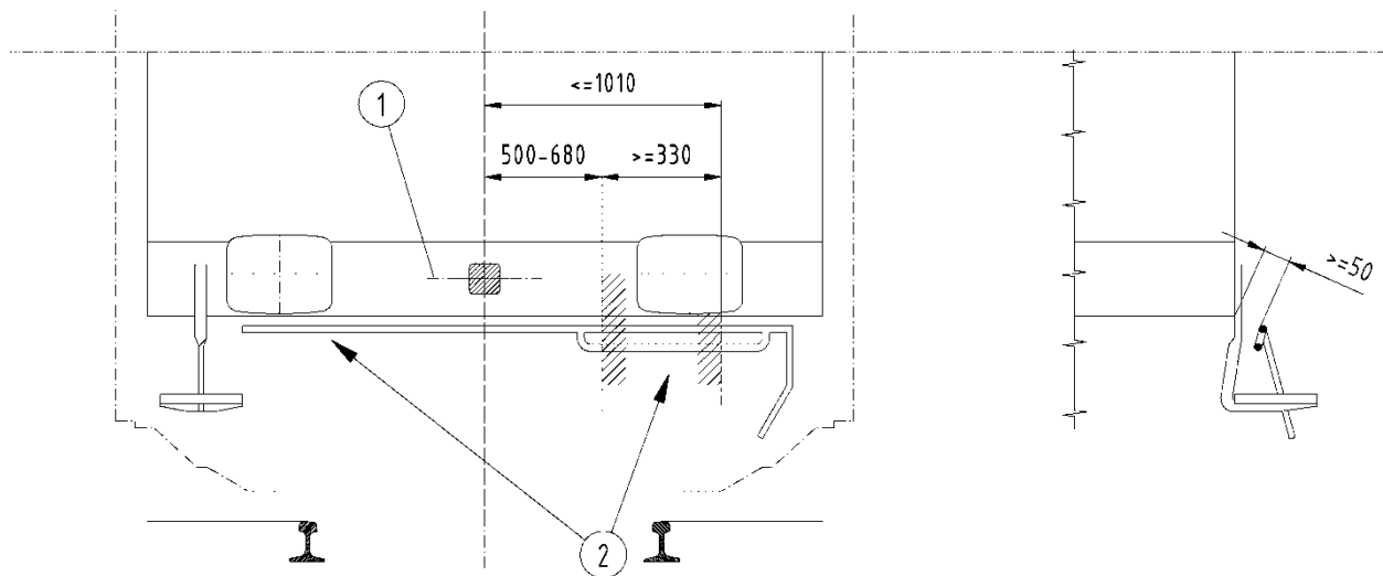
Figure 8: Position of shunter handrails by using automatic coupler
