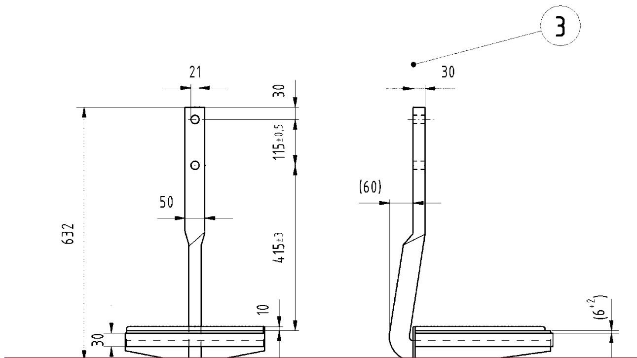
Figure 4: Shunter's step
