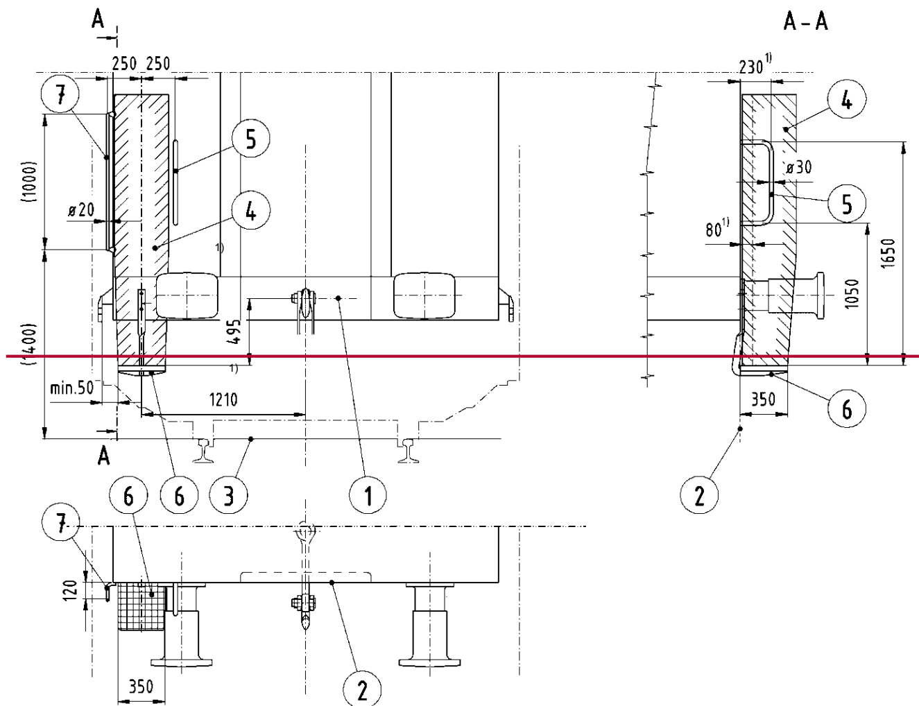
Figure 5: Shunter's stand
