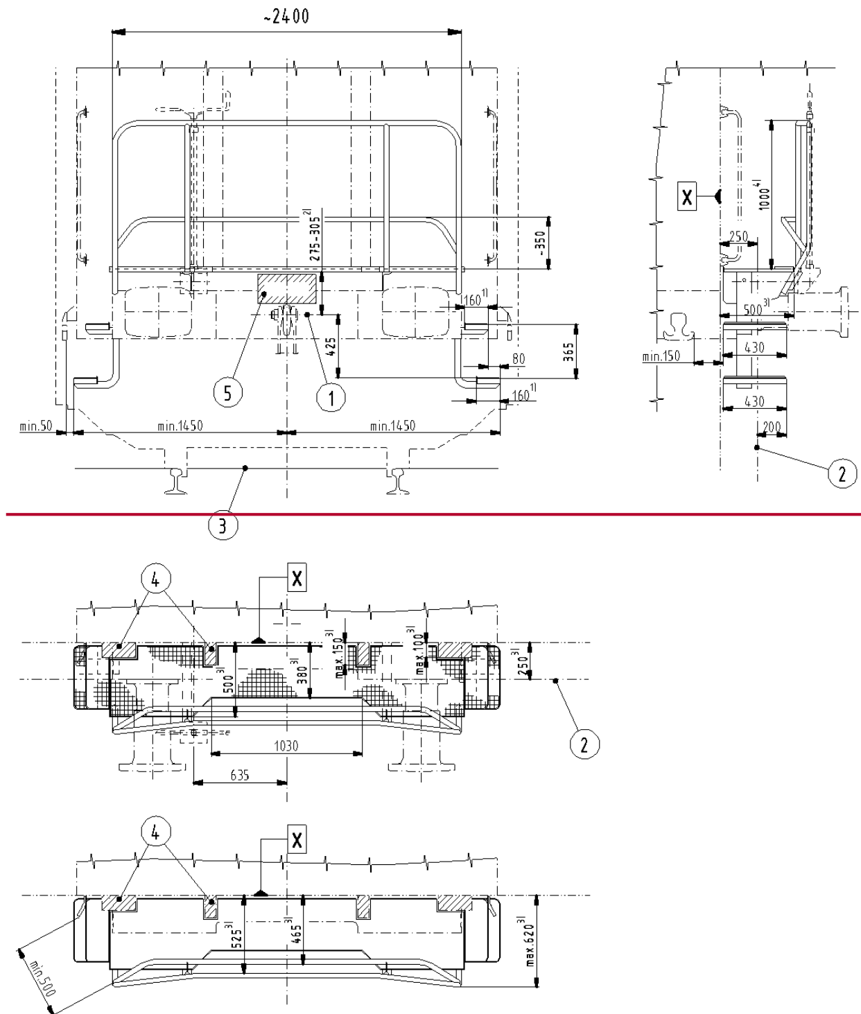
Figure 9: Example for gangway
