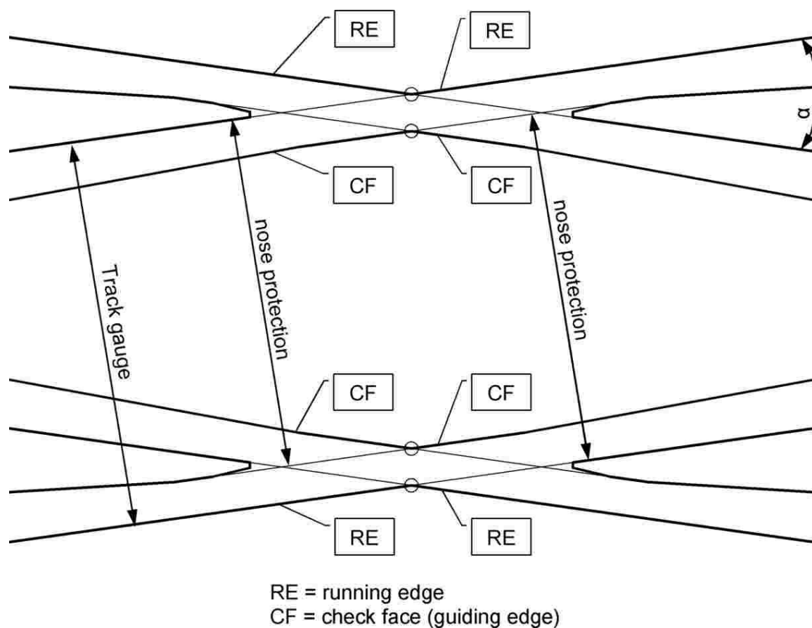
Figure 6 Obtuse crossing
