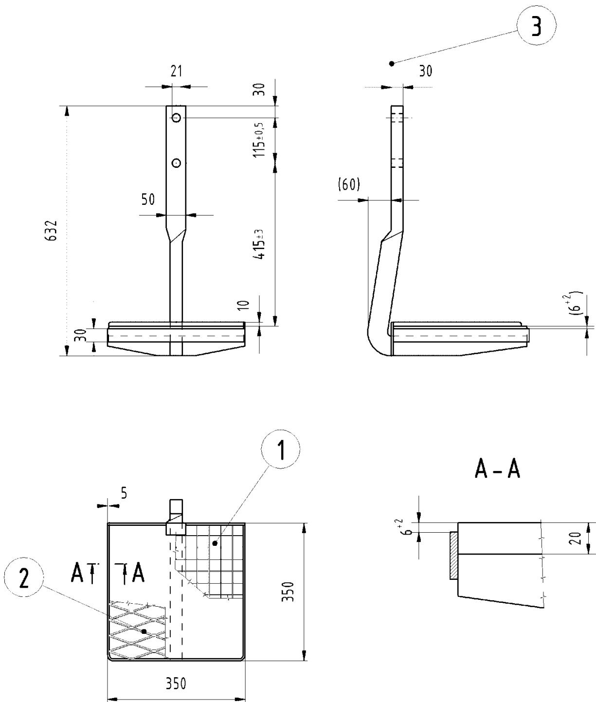
Figure 4: Shunter's step
