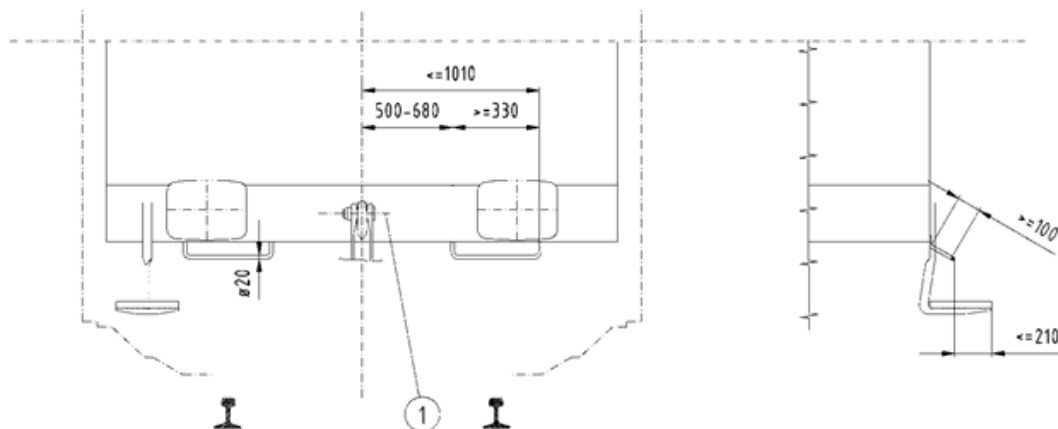
Figure 7: Positions of shunter handrails
