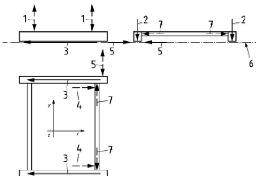
Figure K.2 Overview of transmission of force
