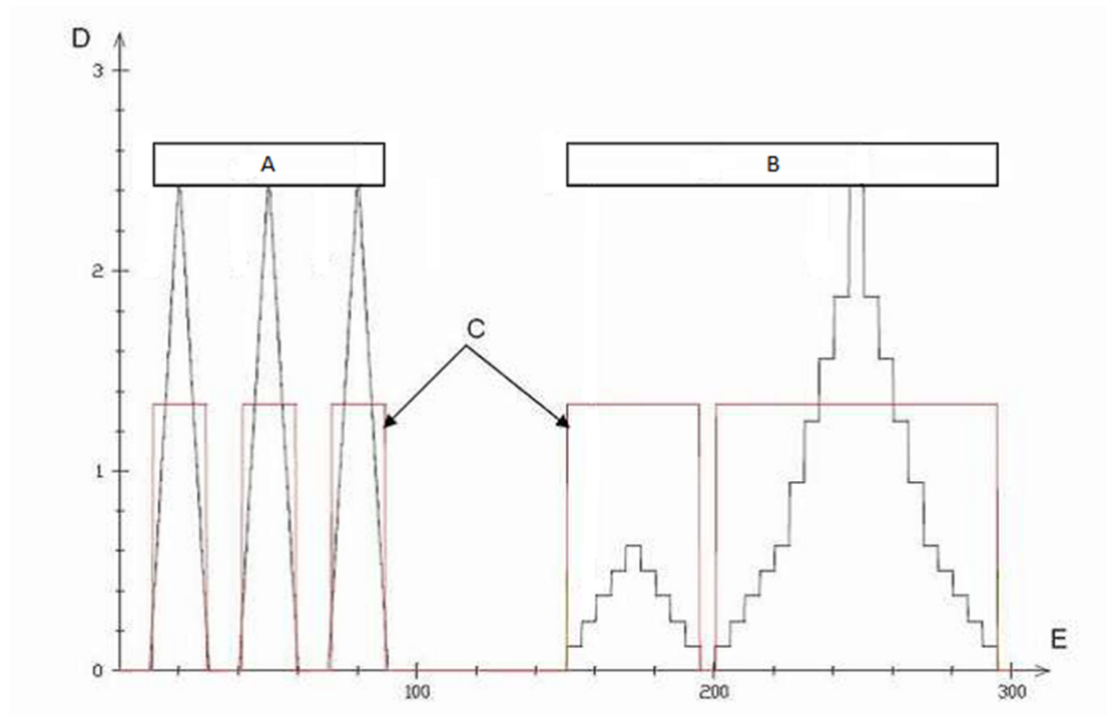
Figure 7: Electrical cycle
