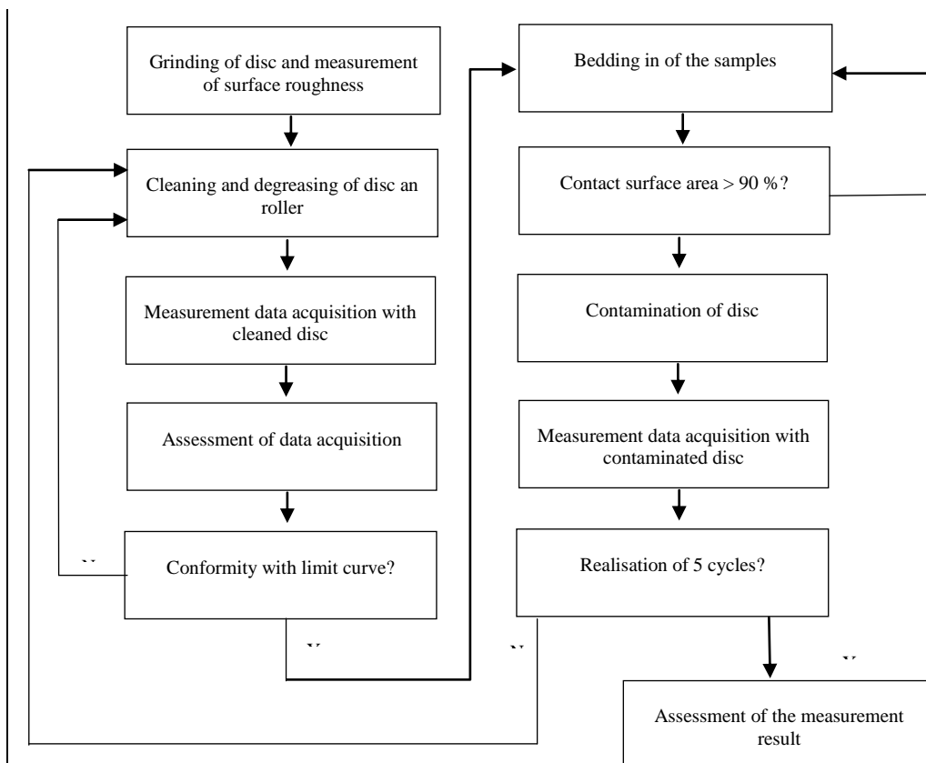
Figure 4: Flow chart of the test program
