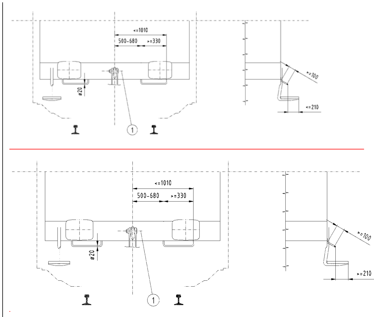
Figure 7: Positions of shunter handrails
