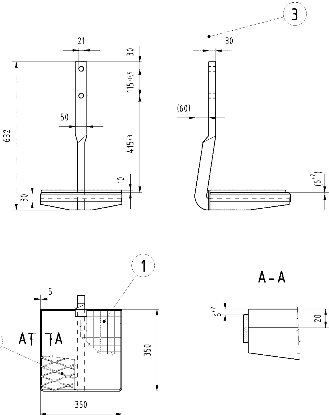
Figure 4: Shunter's step
