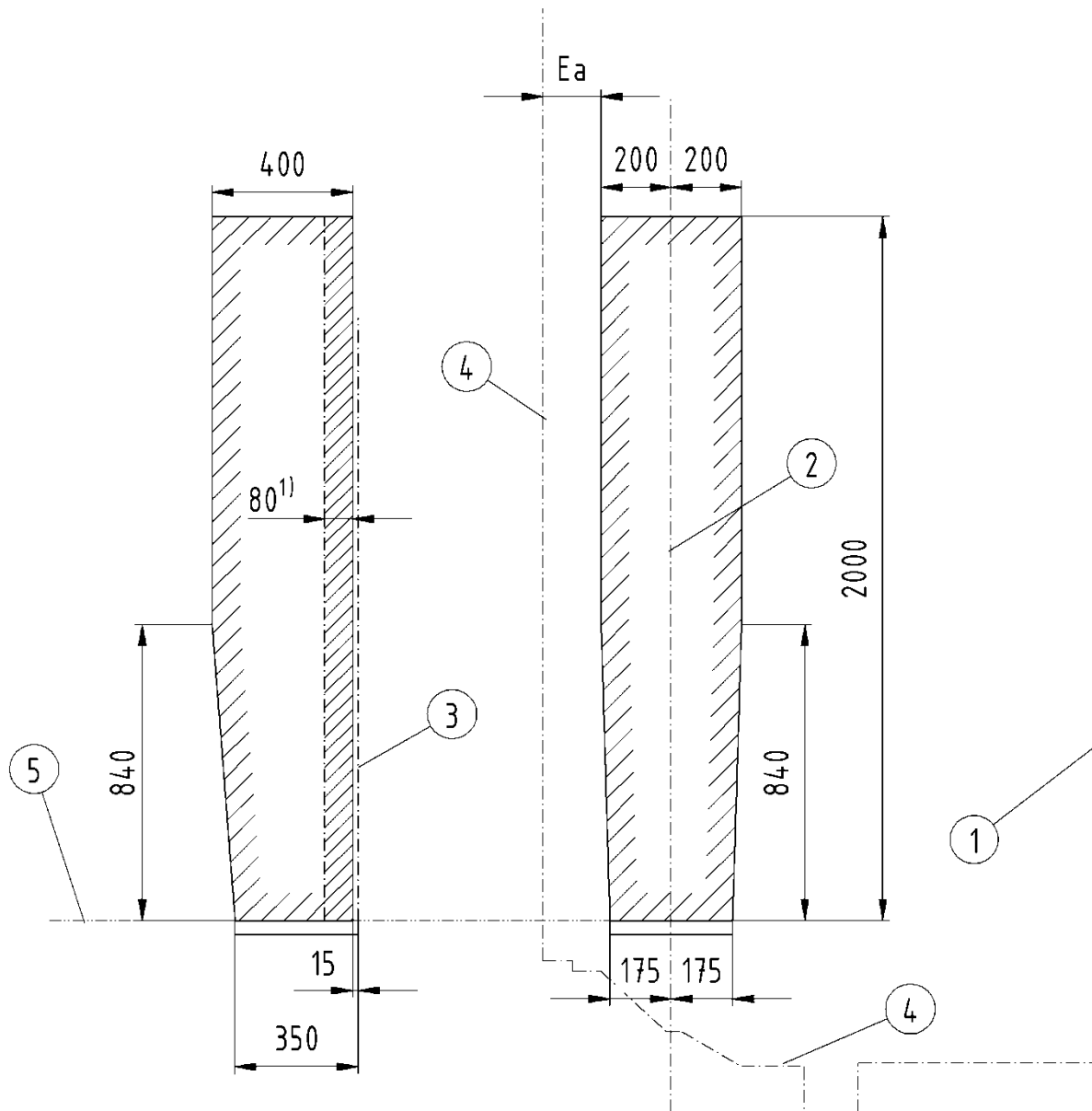
Figure 6: Required space above left footstep
