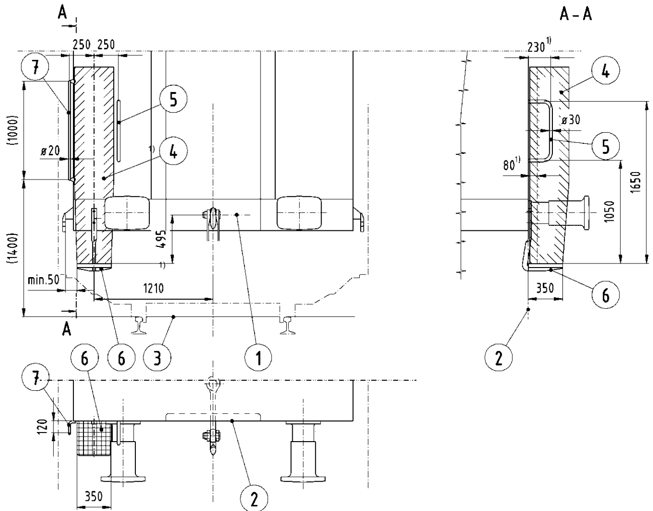
Figure 5: Shunter's stand
