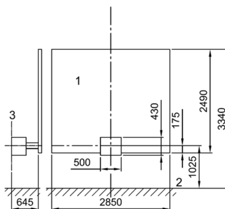
Figure D.1 — Wagon interface with centre coupler (Dimensions in millimetres)
