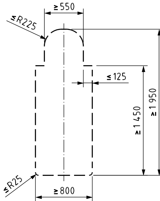
Figure J2 - Minimum clearway profile between connecting vehicles of a single trainset
