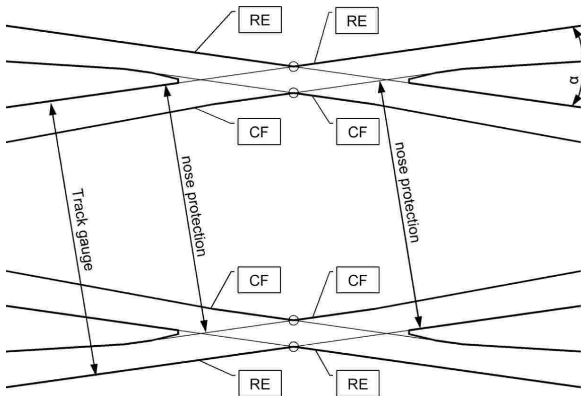
Figure 6 Obtuse crossing
