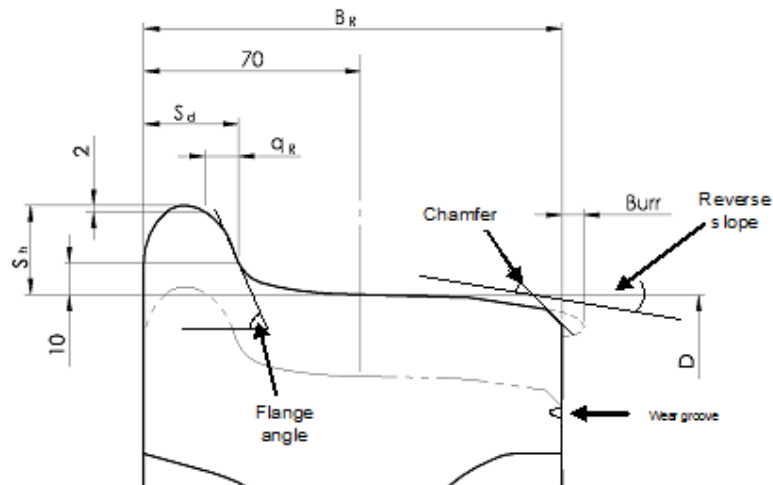
Figure- 2 Symbols for wheels used in table 4
