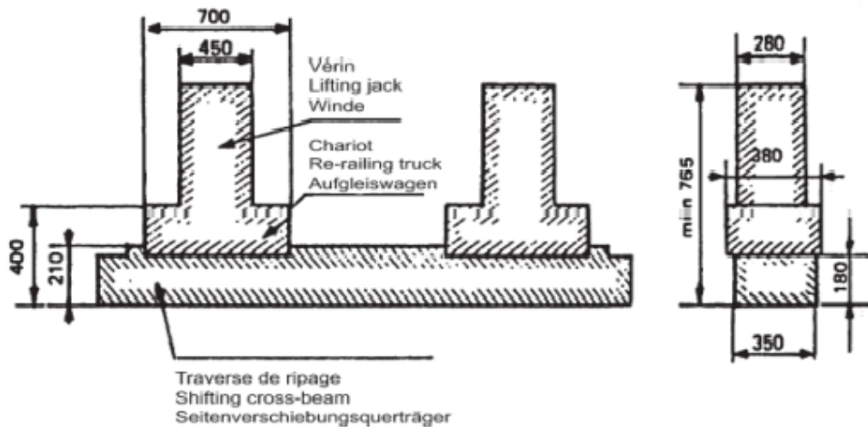
Figure C.2 Free spaces under rerailing places
