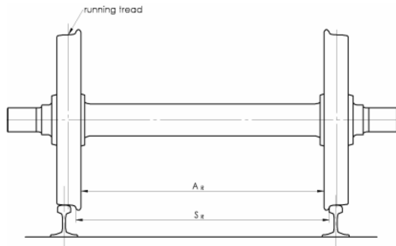
Figure 1 Symbols for wheelsets used in table 3
