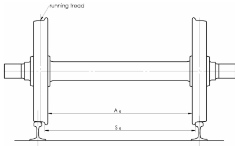
Fig. 1 Symbols for wheelsets used in table 3
