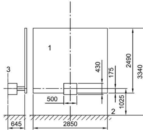
Figure D.1 — Wagon interface with centre coupler
